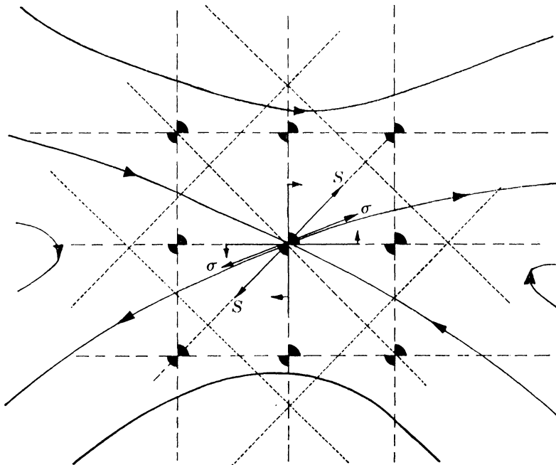
FIGURE 1. Streamlines ( \longrightarrow ), lines of curvature ( - - - ) and strain rate trajectories ( - \cdot - \cdot - ) near a hyperbolic critical point. Extending quadrants are shaded ( \cdot ) and the directions of extension and rotation of fluid lines are marked with light arrows. S is the principal strain rate and \sigma the persistent strain rate.
