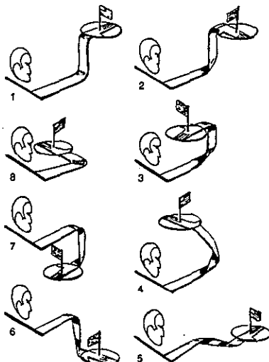
The plate trick — illustrating a geometrical principle popularized by Dirac, explained by Newman with the theory of braid groups.
