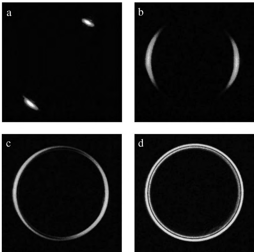
Fig. 5. The transition (a–d) from double to conical refraction as the incident beam direction approaches the optic axis. In (d) two rings are visible, separated by the Poggendorff dark ring studied in Section 5. This figure is taken from Berry, Jeffrey and Lunney [2006] (see also Table 1).
