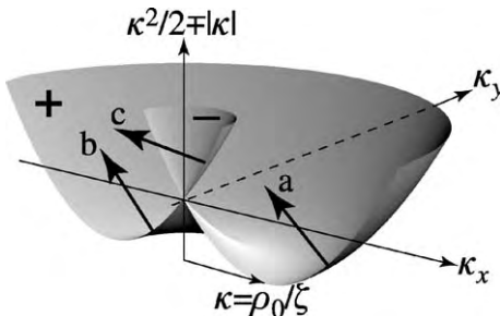
Fig. 8. The 'Hamiltonian' surface (5.10) whose normals generate the paraxial rays.
