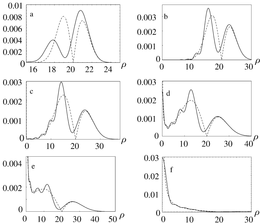
Fig. 12. Intensity for a Gaussian incident beam for \rho_0 = 20 and (a) \zeta = 1 ; (b) \zeta = 4 ; (c) \zeta = 6 ; (d) \zeta = 8 ; (e) \zeta = 10 ; (f) \zeta = 20 . Solid curves: exact theory; dashed curves: refined geometrical-optics theory (7.13).
