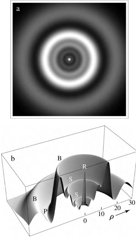
Fig. 13. (a) Density plot and (b) cutaway 3D plot, of conical diffraction intensity for \rho_0 = 20 , \zeta = 8 , showing bright rings B, Poggendorff dark ring P, Raman spot R and secondary rings S.
