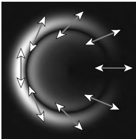
Fig. 6. Simulation of rings for incident beam linearly polarized horizontally, with polarization directions superimposed, showing the ‘fermionic’ half-turn of the polarization.
