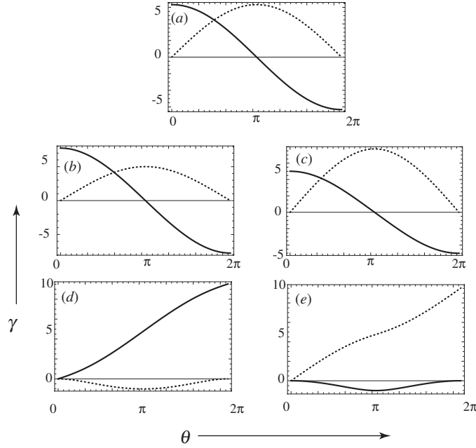
Figure 3. \text{Re } \gamma(\theta) (full curves) and \text{Im } \gamma(\theta) (dotted curves) for (a) degeneracy-centred loop \rho = 10, R = 0 ; eccentric degeneracy-enclosing loops (b) \rho = 10, R = 4.3 , (c) \rho = 10, R = -4.3 ; eccentric degeneracy-excluding loops (d) \rho = 1.5, R = 2.3 , (e) \rho = 1.5, R = -2.3 .
